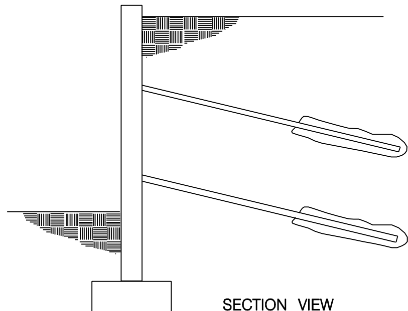
SECTION VIEW
