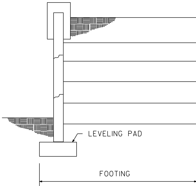
SECTION VIEW
